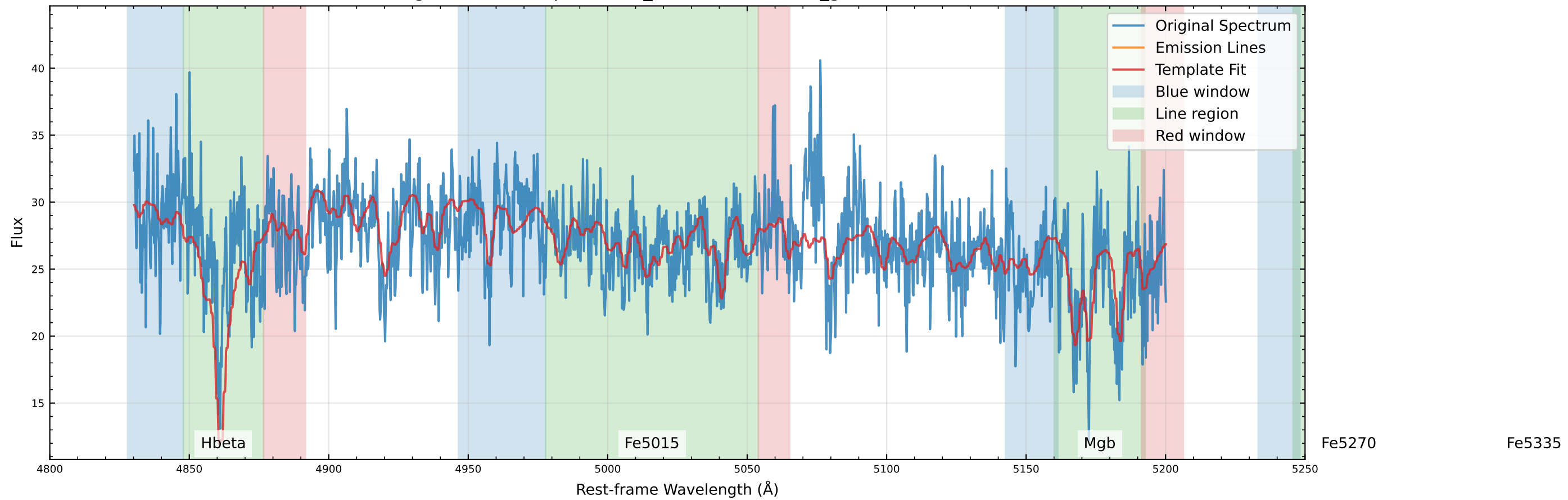
Original Data Comparison (v_star=-20.2 km/s, v_gas=-9.0 km/s)
