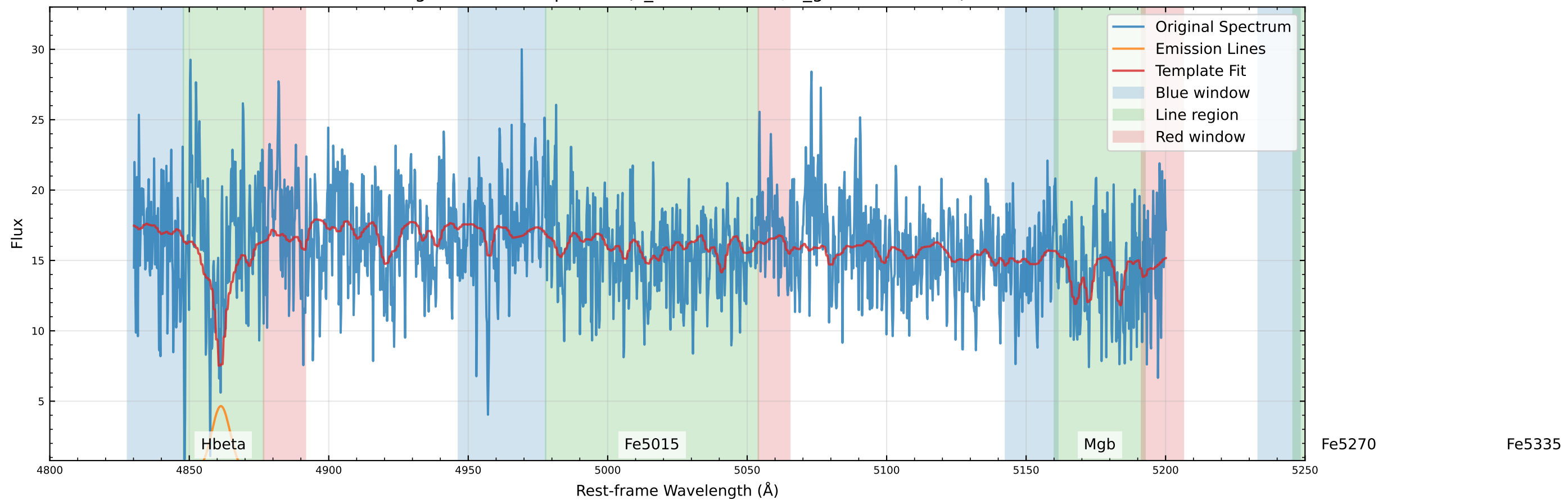
Original Data Comparison (v_star=0.5 km/s, v_gas=207.1 km/s)
