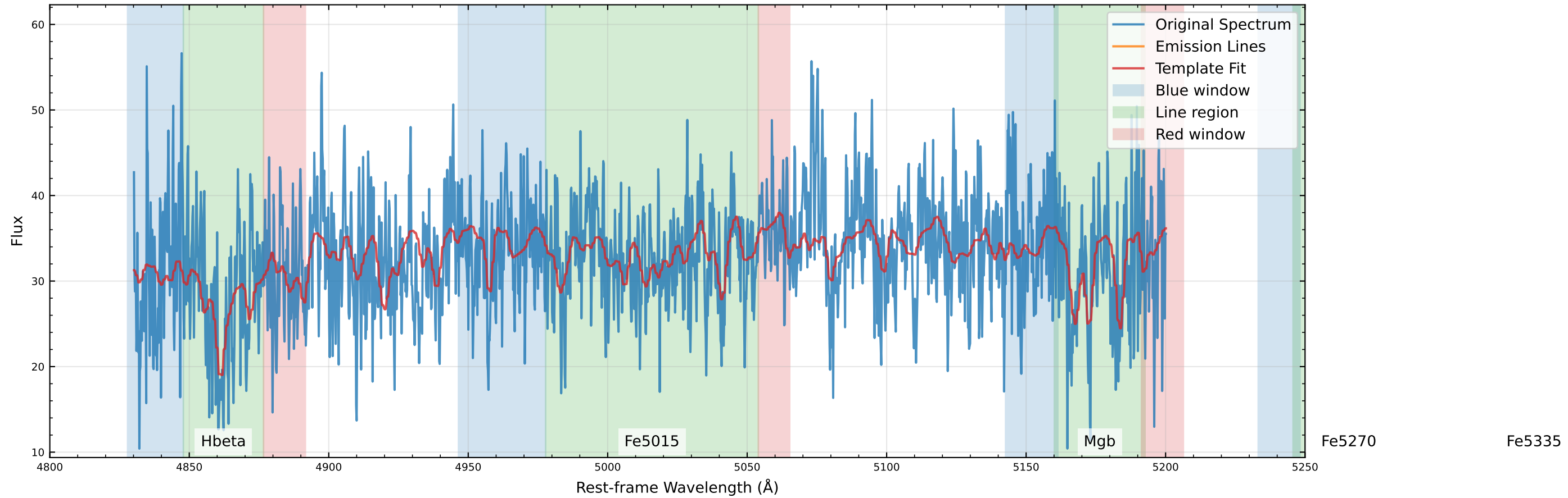
Original Data Comparison (v_star=-26.2 km/s, v_gas=-5.5 km/s)
