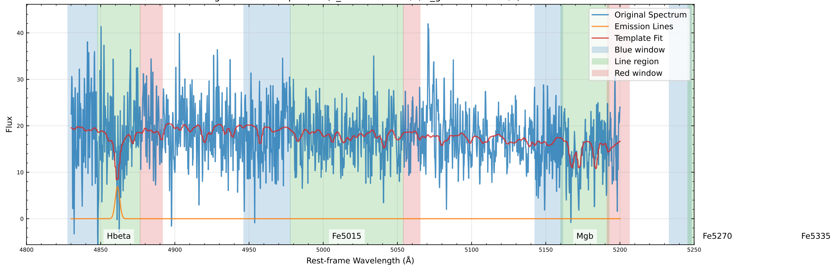
Original Data Comparison (v_star=-25.6 km/s, v_gas=-171.8 km/s)
