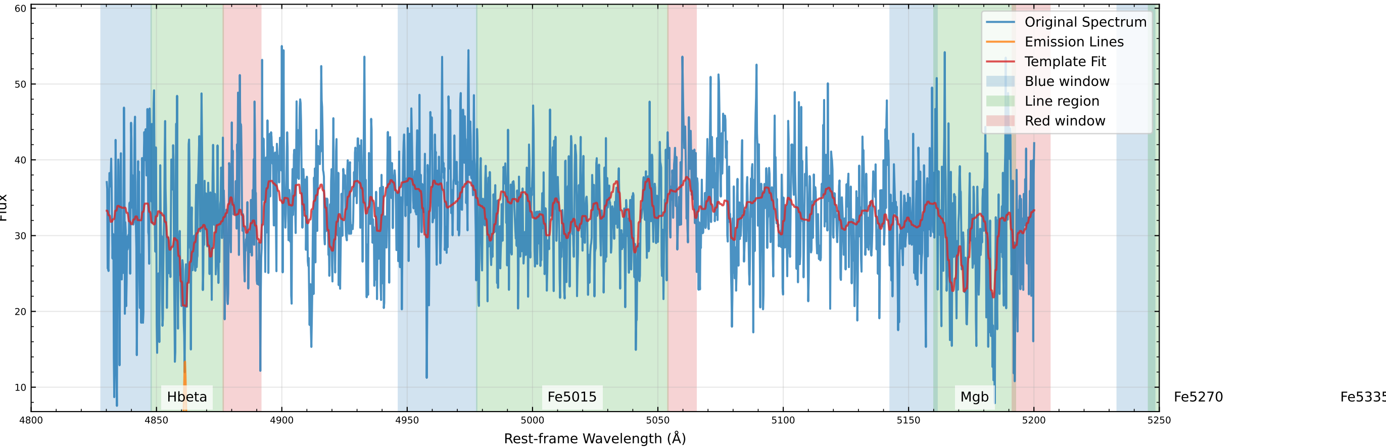
Original Data Comparison (v_star=19.8 km/s, v_gas=97.4 km/s)
