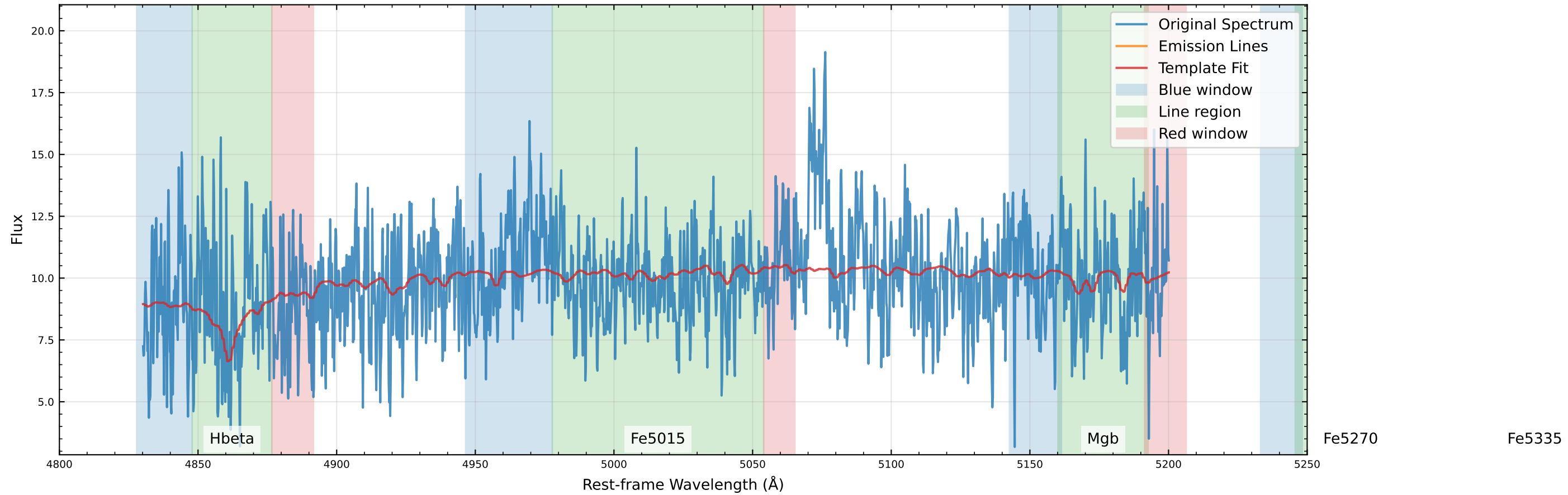
Original Data Comparison (v_star=14.5 km/s, v_gas=74.7 km/s)
