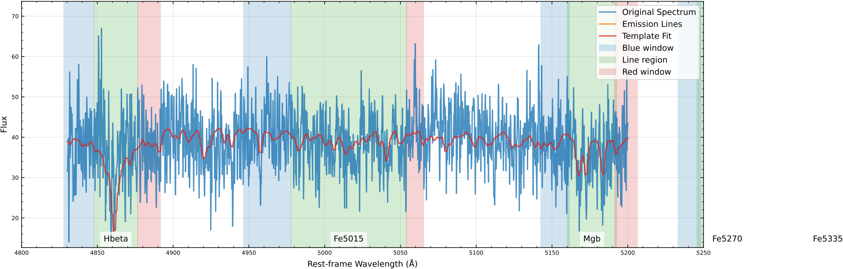
Original Data Comparison (v_star=25.7 km/s, v_gas=130.9 km/s)
