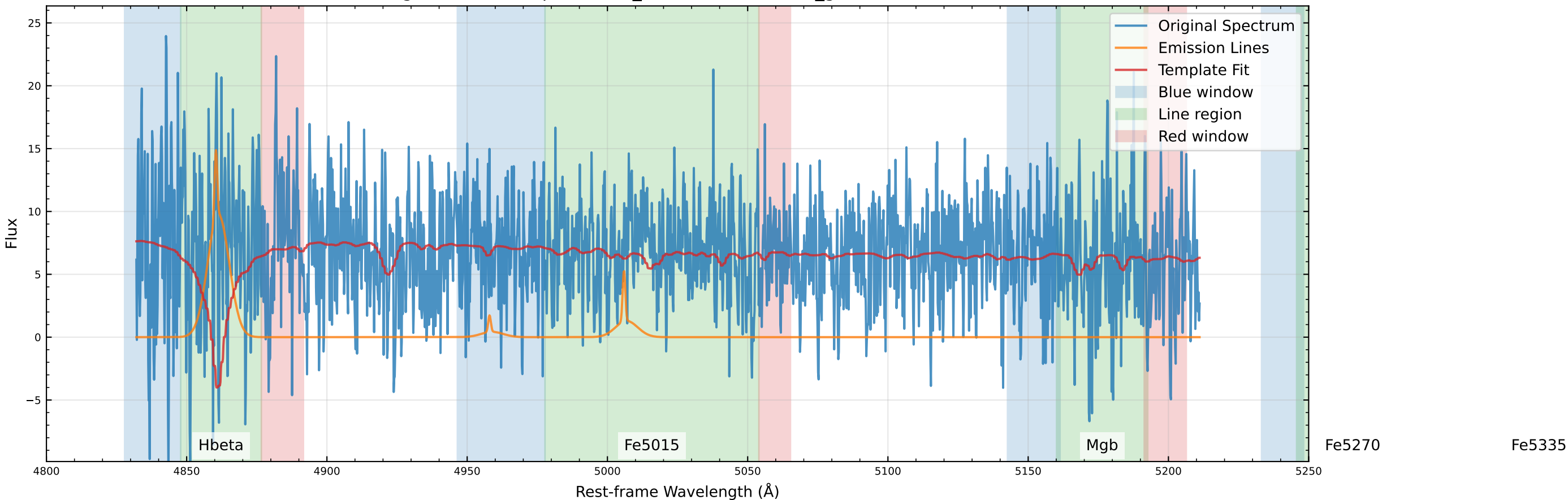
Original Data Comparison (v_star=106.8 km/s, v_gas=133.7 km/s)
