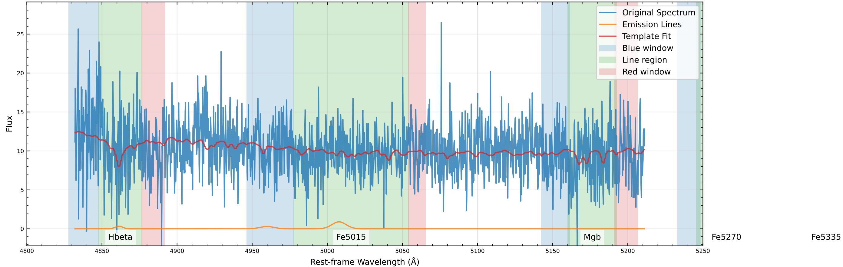
Original Data Comparison (v_star=-22.3 km/s, v_gas=5.3 km/s)
