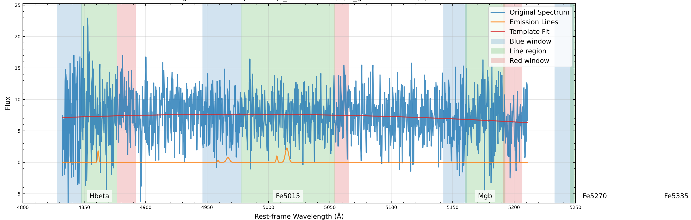
Original Data Comparison (v_star=0.0 km/s, v_gas=-282.7 km/s)
