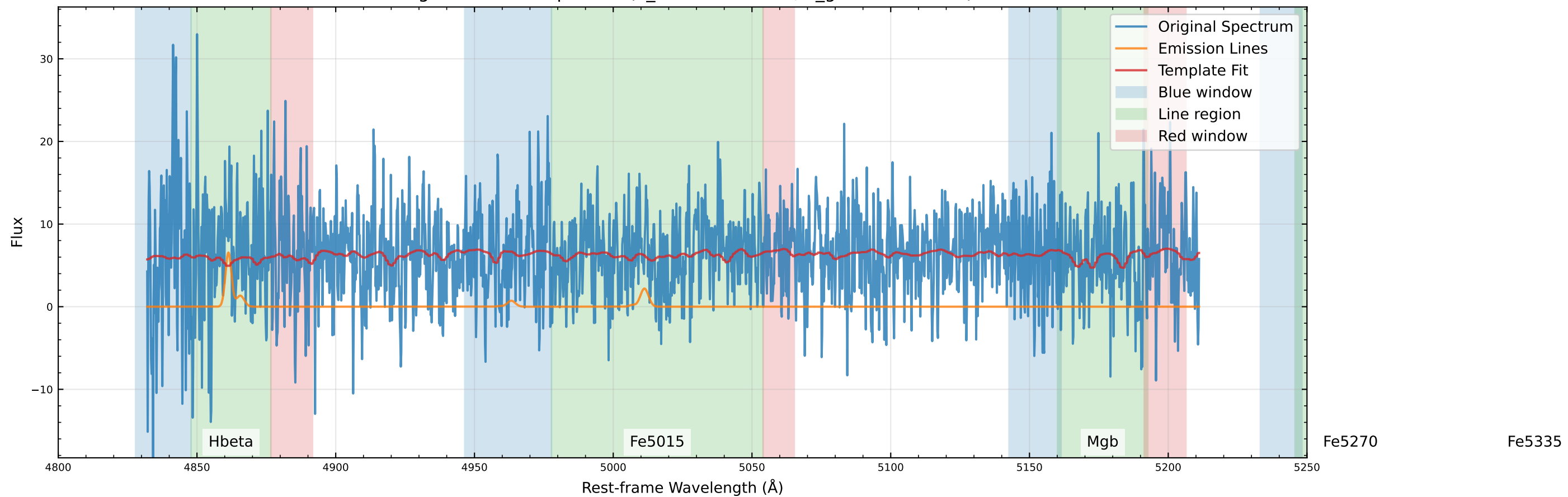
Original Data Comparison (v_star=82.7 km/s, v_gas=-16.7 km/s)
