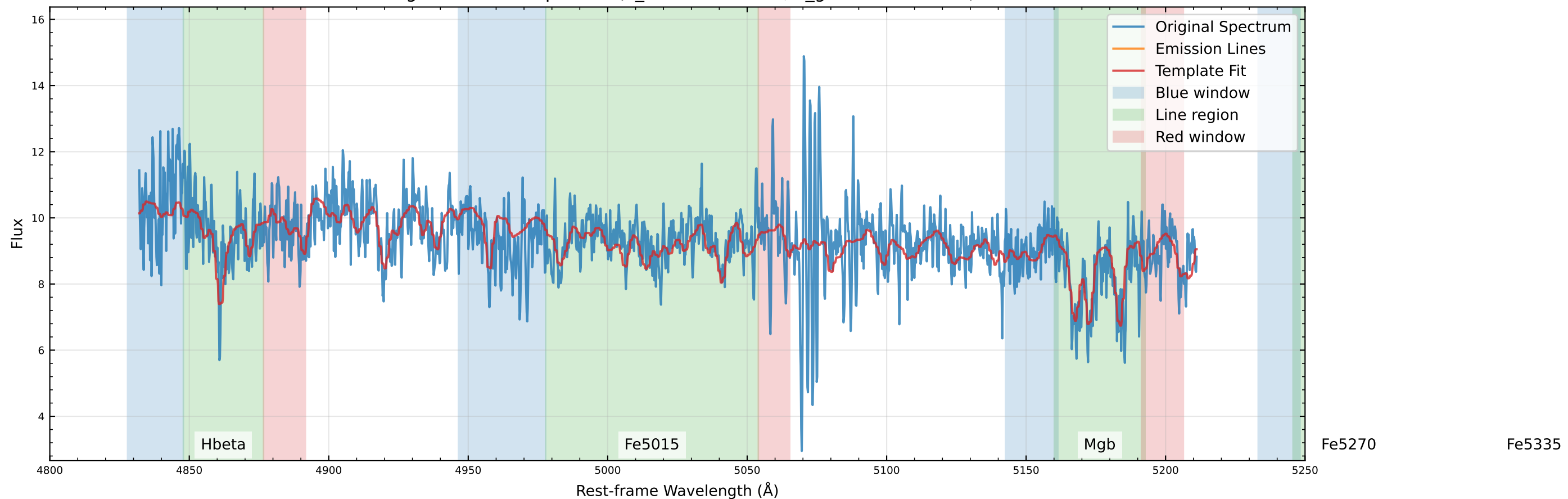
Original Data Comparison (v_star=11.1 km/s, v_gas=-185.6 km/s)
