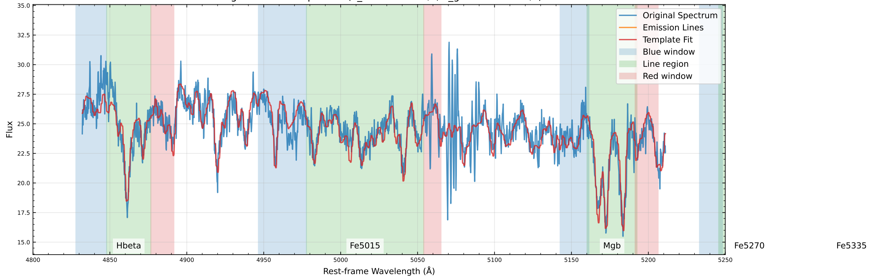
Original Data Comparison (v_star=-6.4 km/s, v_gas=-306.4 km/s)
