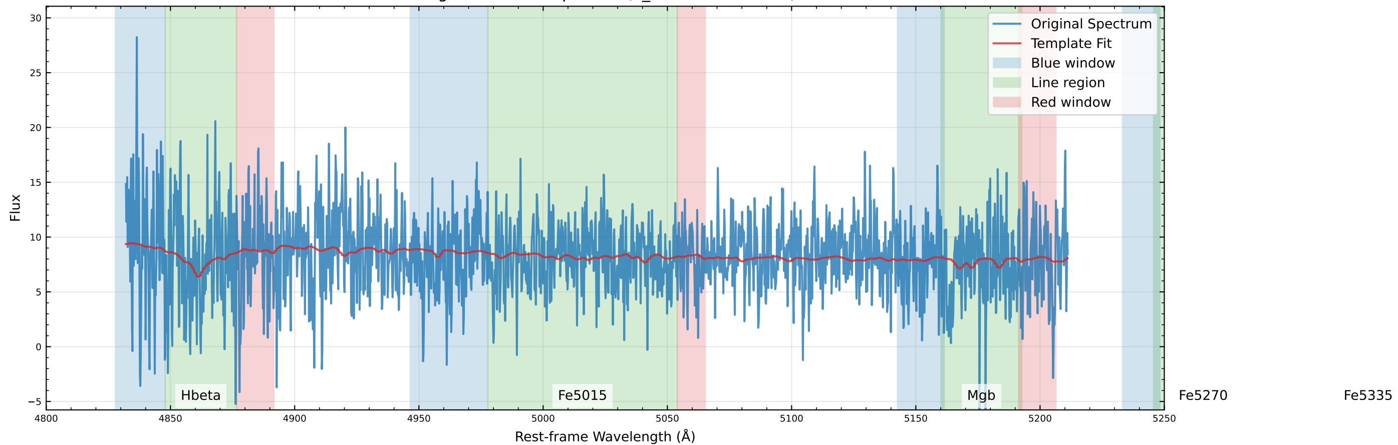
Original Data Comparison (v_star=-328.8 km/s)
