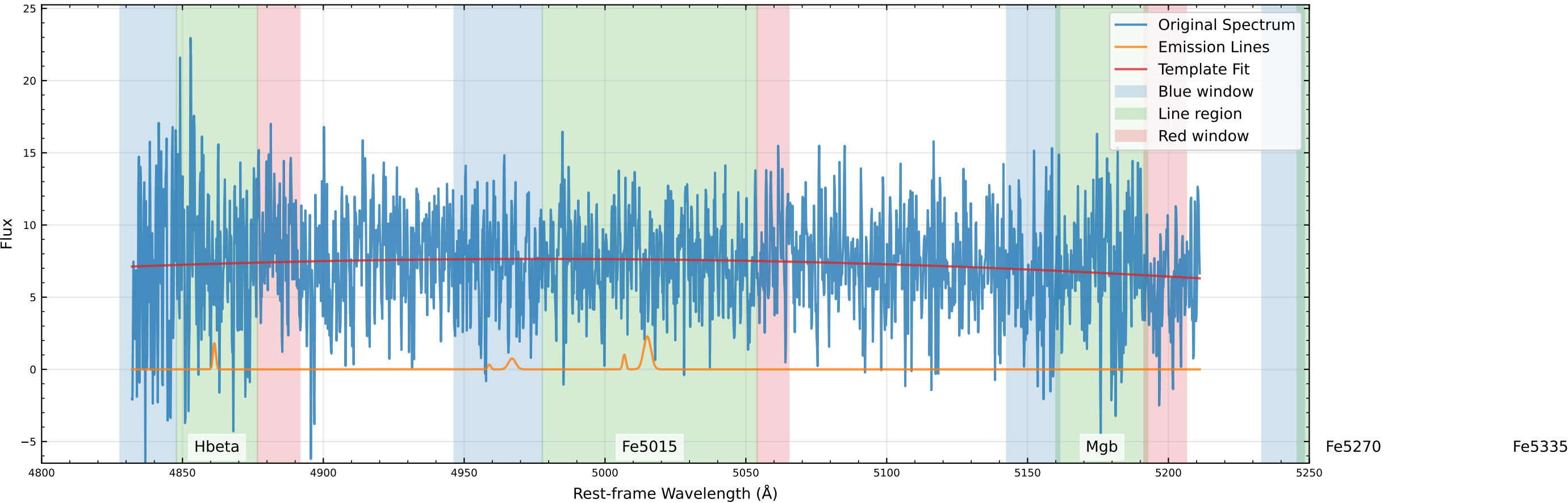
Original Data Comparison (v_star=0.0 km/s, v_gas=-282.7 km/s)
