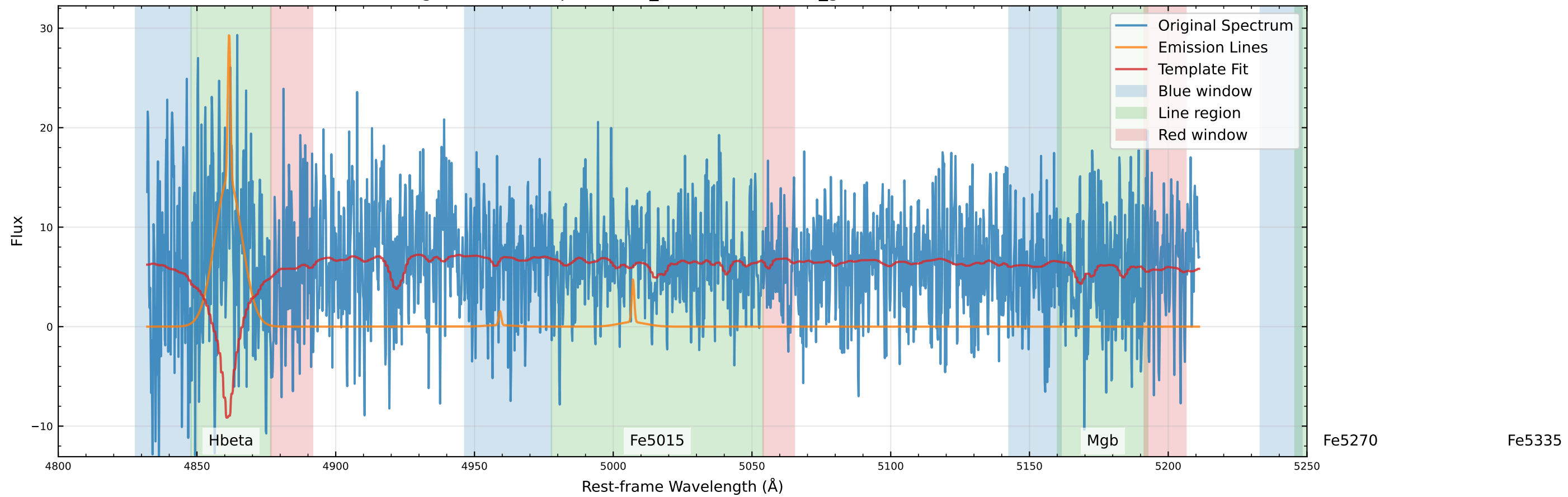
Original Data Comparison (v_star=40.9 km/s, v_gas=33.3 km/s)
