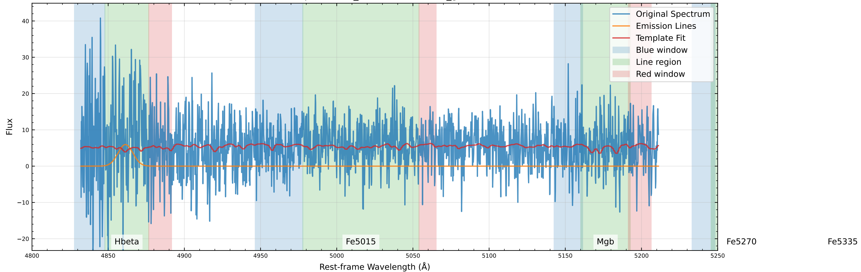
Original Data Comparison (v_star=65.7 km/s, v_gas=365.7 km/s)
