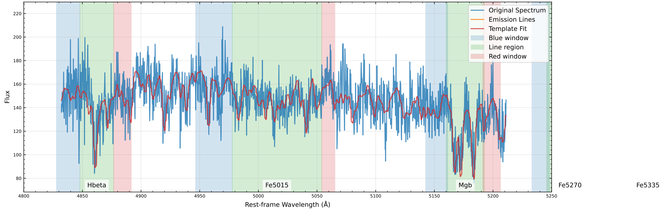
Original Data Comparison (v_star=4.5 km/s)
