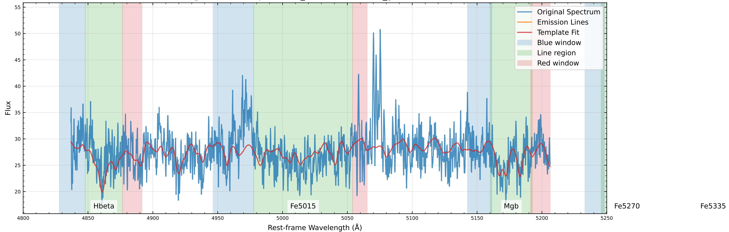
Original Data Comparison (v_star=-18.8 km/s, v_gas=1.8 km/s)
