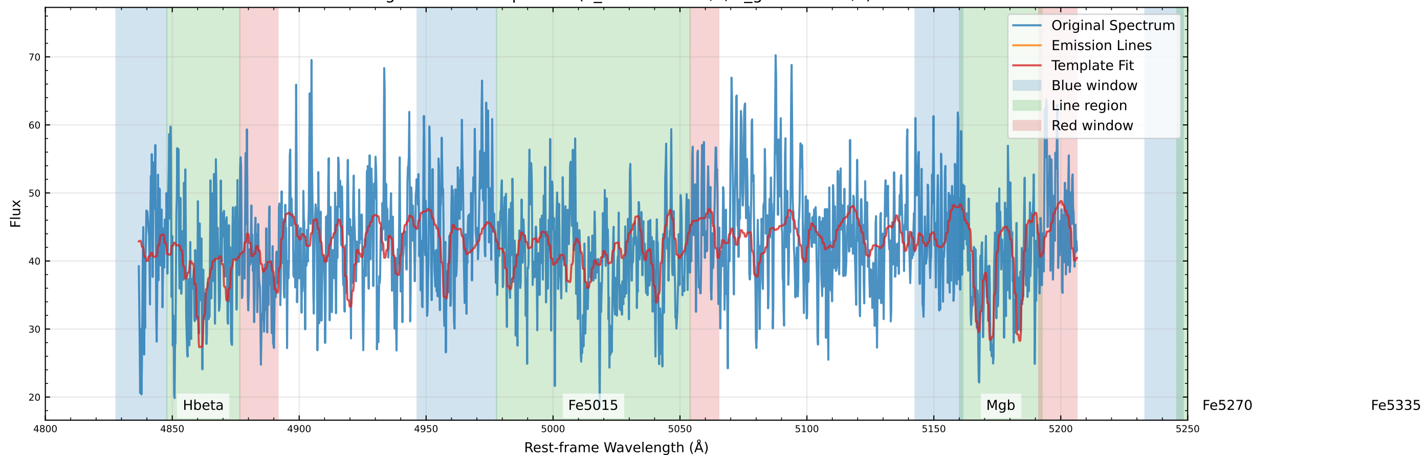
Original Data Comparison (v_star=-0.2 km/s, v_gas=6.4 km/s)
