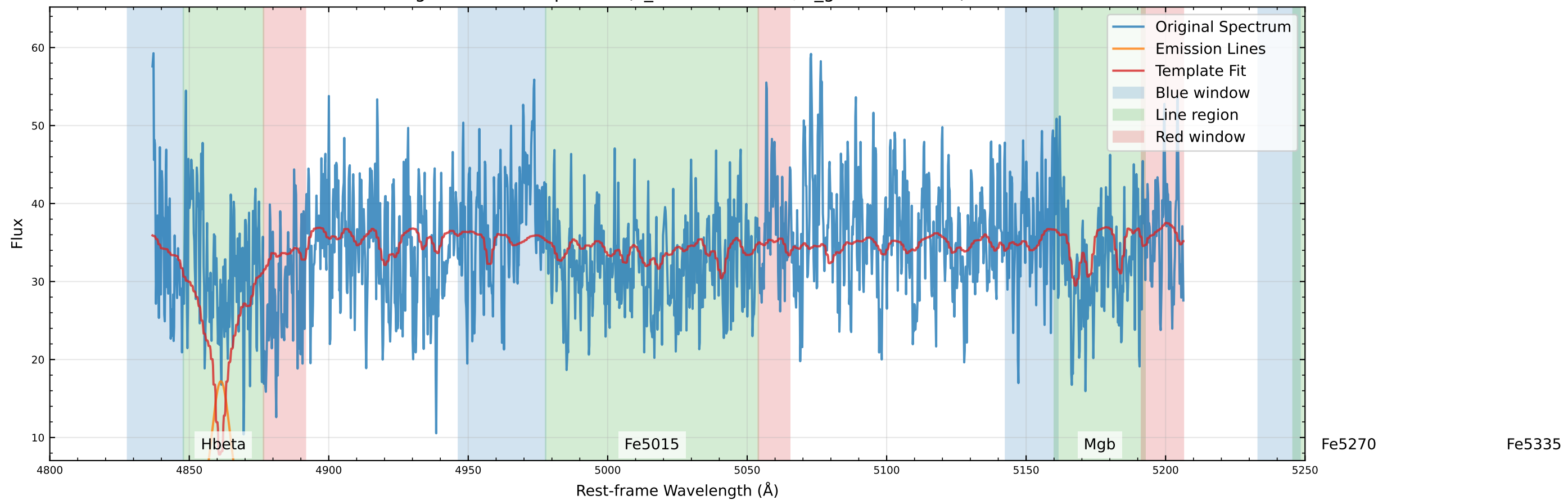
Original Data Comparison (v_star=56.1 km/s, v_gas=85.3 km/s)
