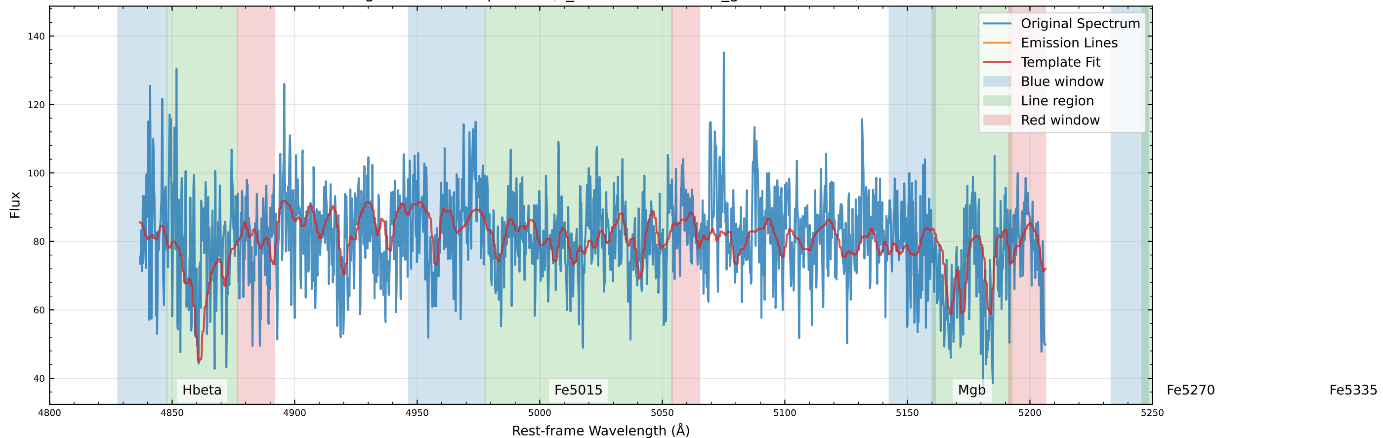
Original Data Comparison (v_star=-63.7 km/s, v_gas=-30.4 km/s)
