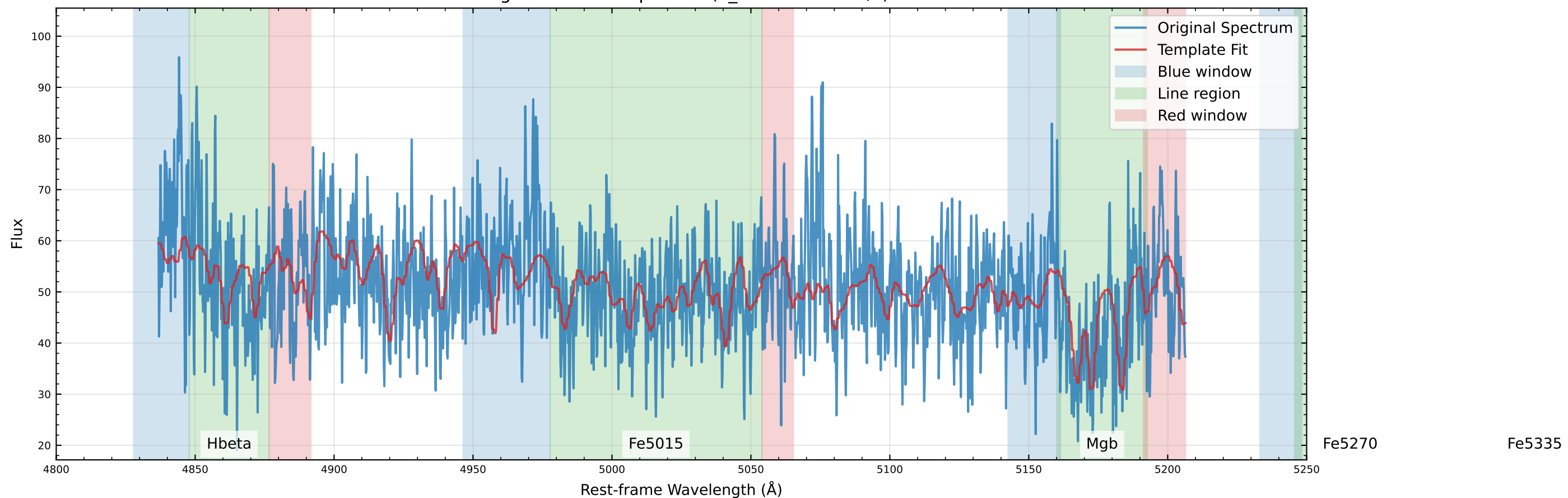
Original Data Comparison (v_star=-20.8 km/s)
