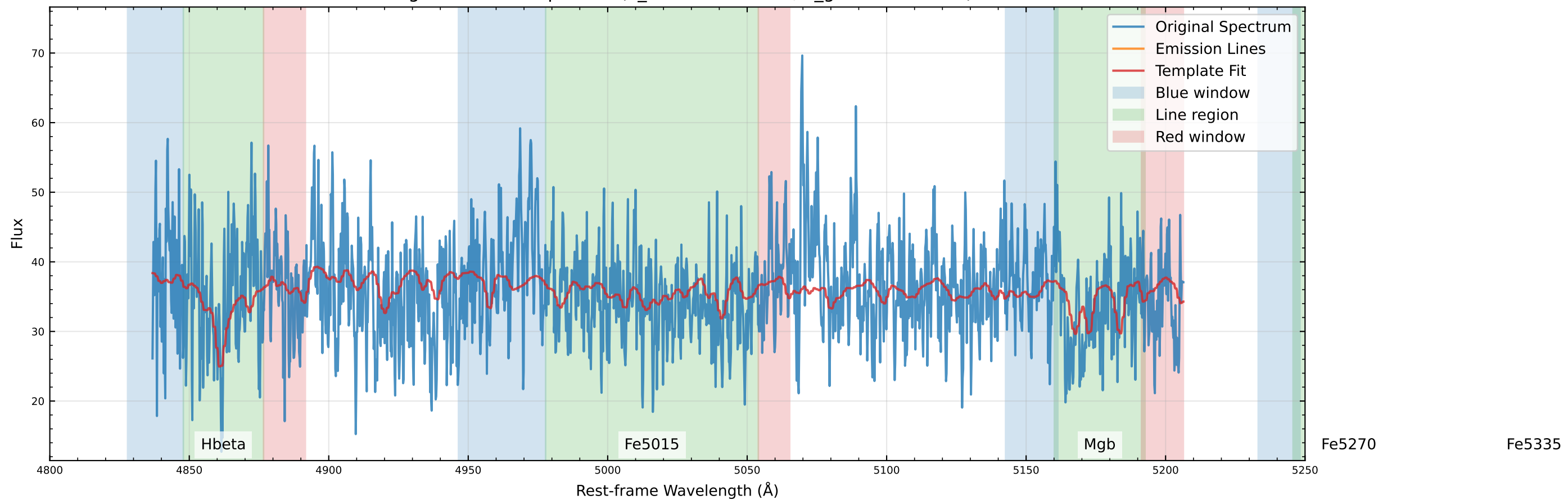
Original Data Comparison ( v_{\text{star}}=-76.1 km/s, v_{\text{gas}}=-92.8 km/s)
