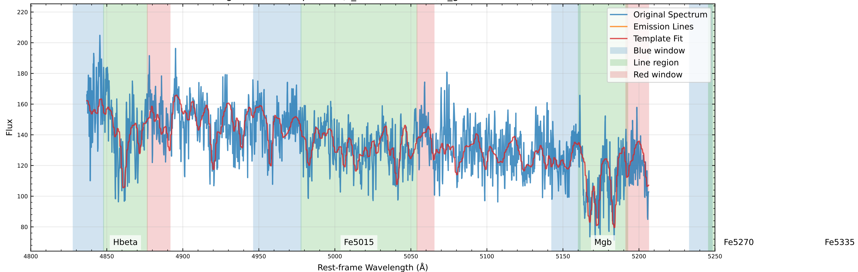
Original Data Comparison (v_star=-39.0 km/s, v_gas=-65.8 km/s)
