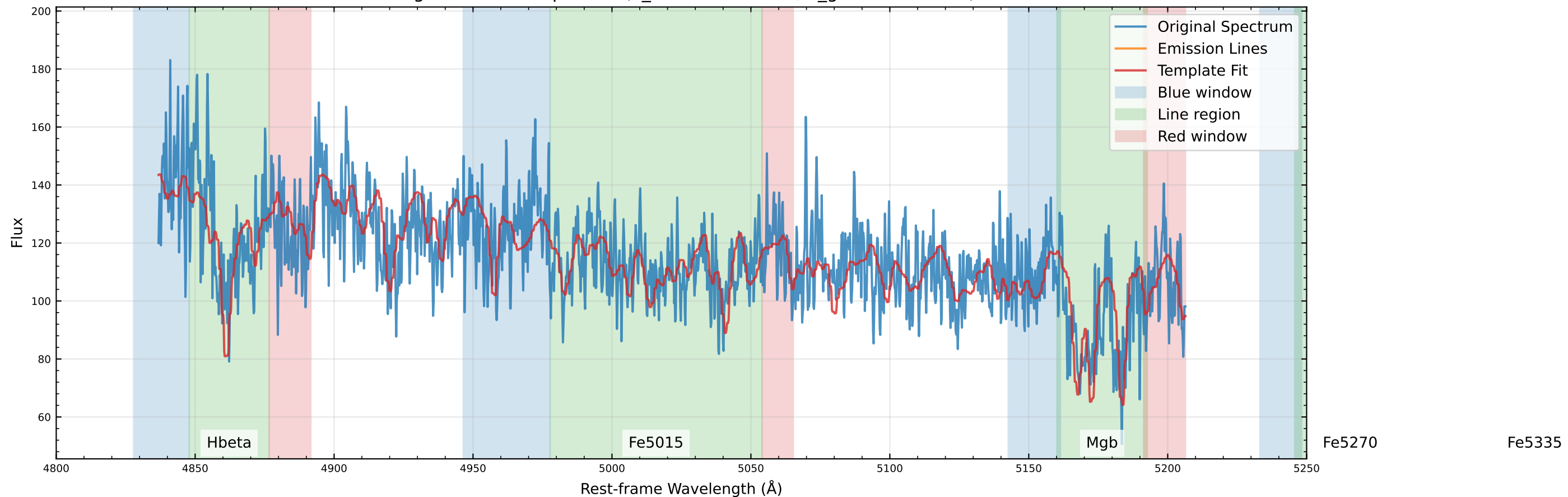
Original Data Comparison (v_star=-53.8 km/s, v_gas=-78.8 km/s)
