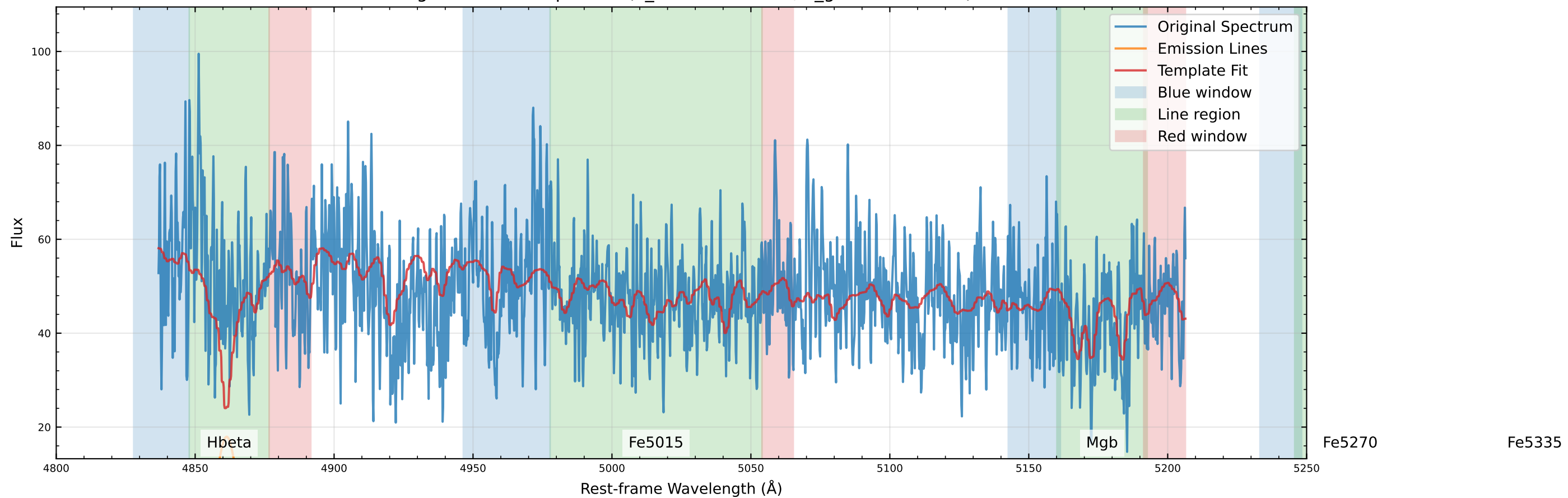
Original Data Comparison (v_star=18.8 km/s, v_gas=-12.4 km/s)
