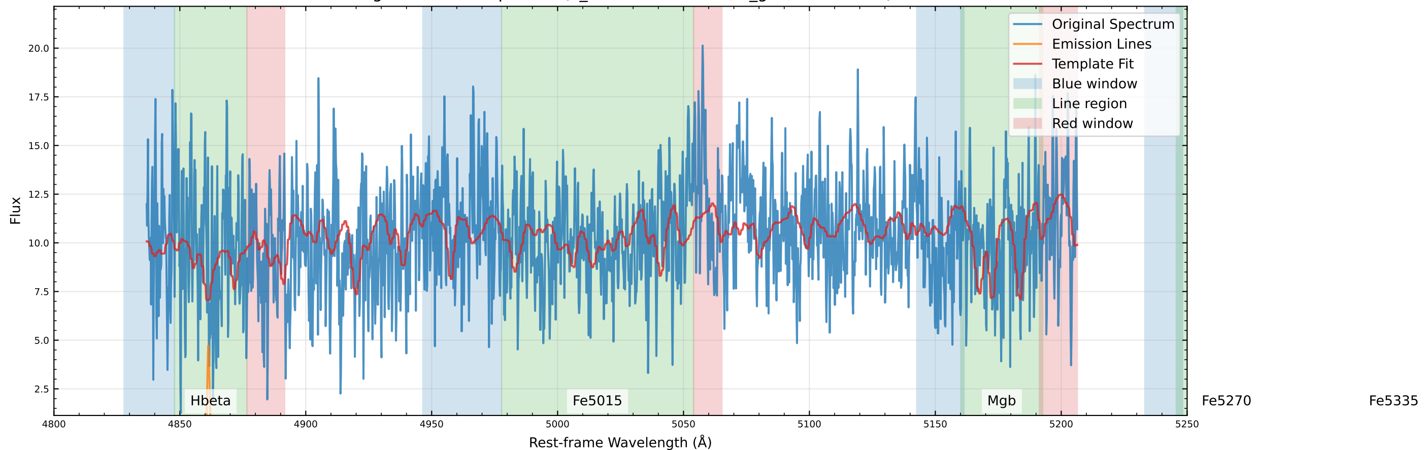
Original Data Comparison (v_star=-131.7 km/s, v_gas=-84.1 km/s)
