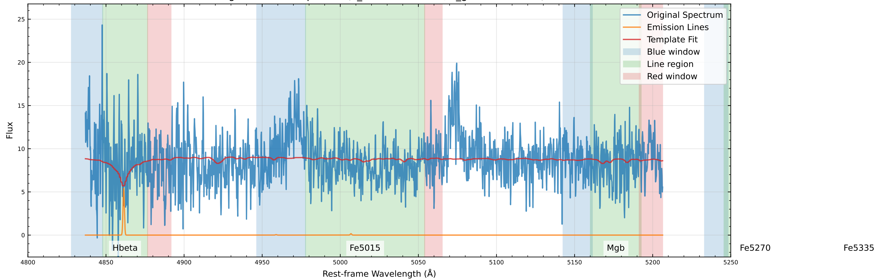
Original Data Comparison (v_star=-68.1 km/s, v_gas=-82.0 km/s)
