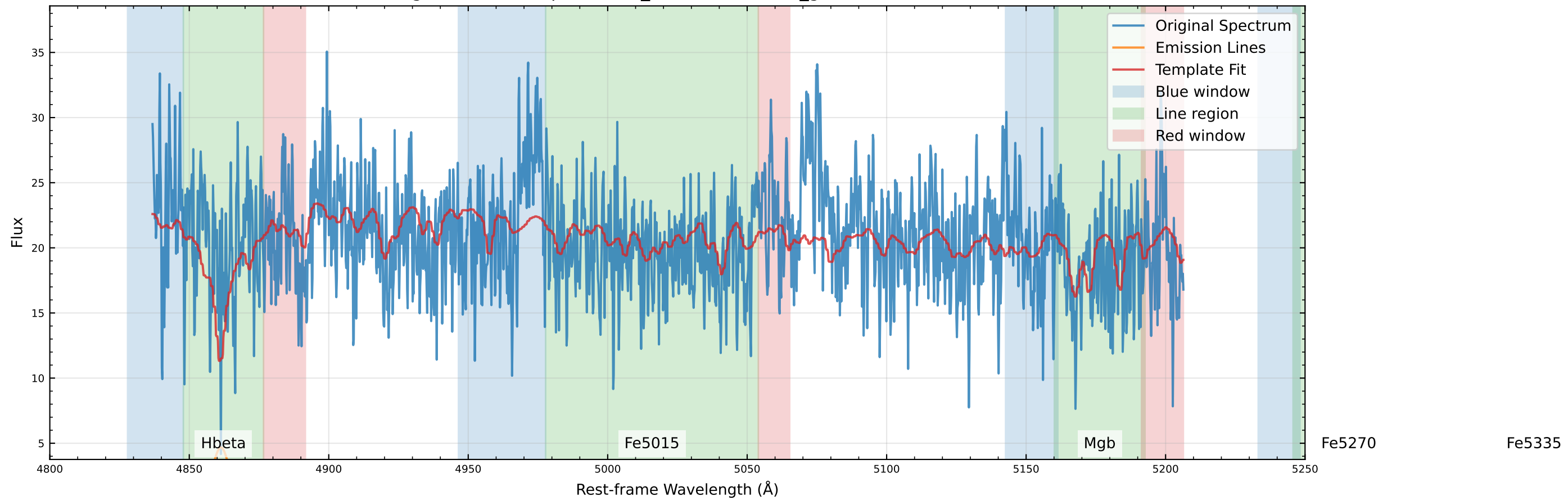
Original Data Comparison (v_star=0.7 km/s, v_gas=-214.3 km/s)
