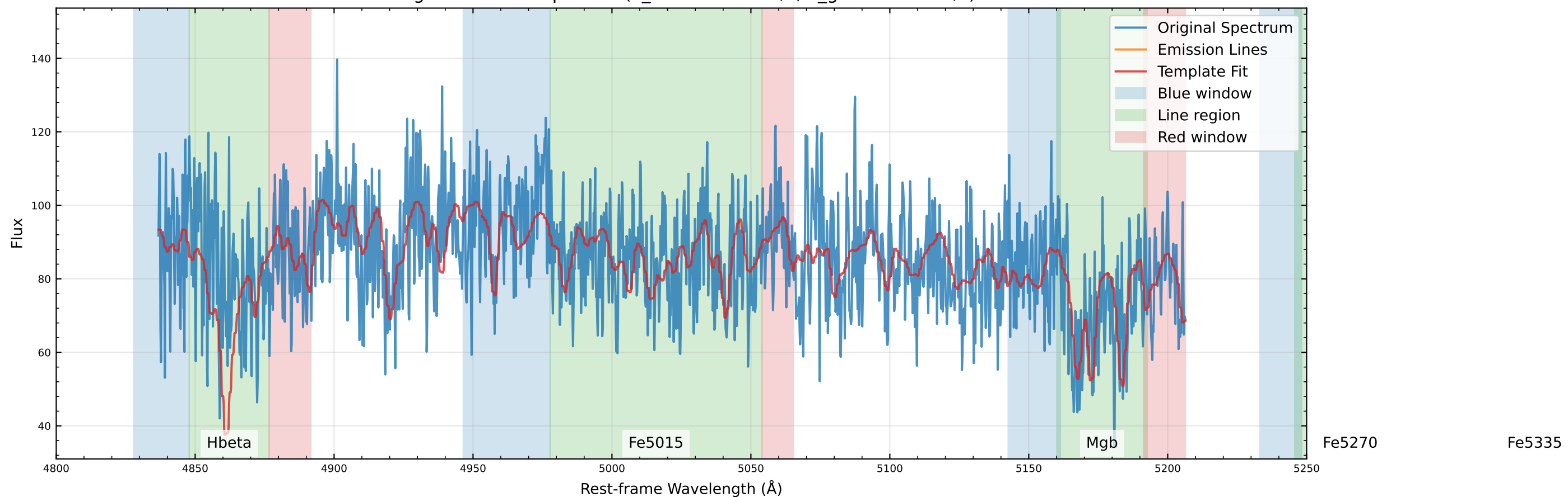
Original Data Comparison (v_star=-13.0 km/s, v_gas=-62.5 km/s)
