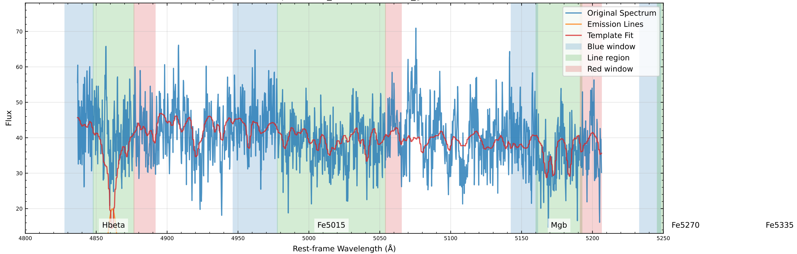
Original Data Comparison (v_star=-4.5 km/s, v_gas=-87.9 km/s)
