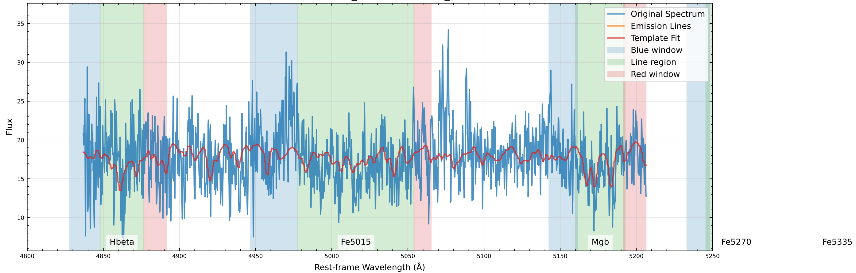
Original Data Comparison (v_star=75.2 km/s, v_gas=49.5 km/s)
