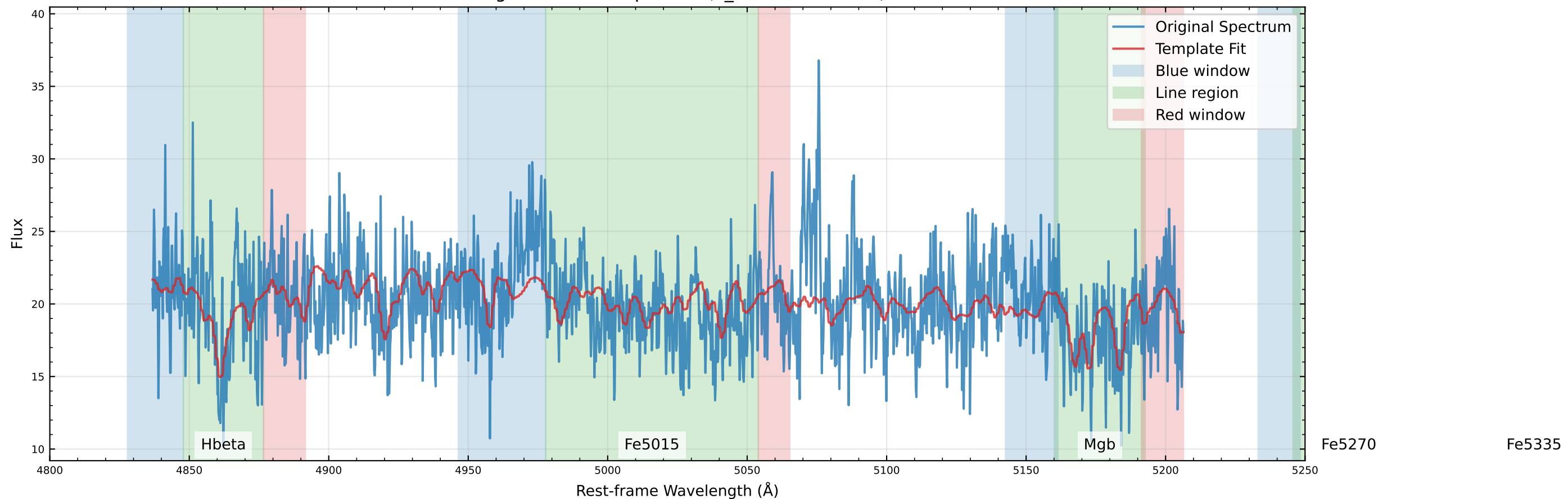
Original Data Comparison (v_star=-11.6 km/s)
