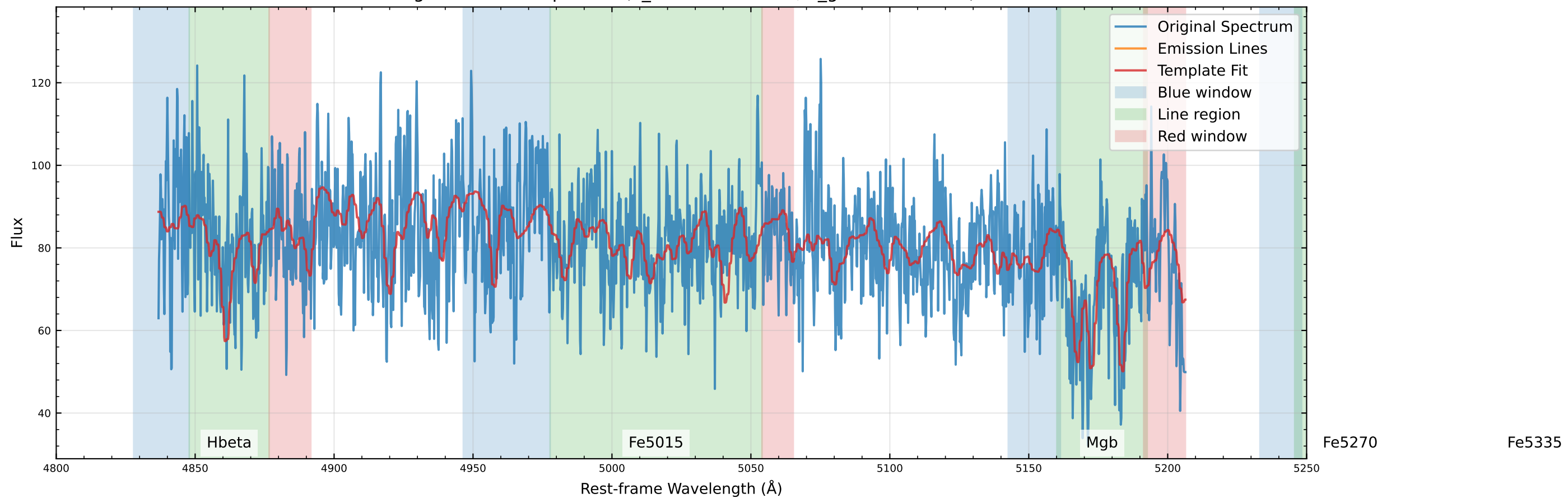
Original Data Comparison (v_star=-66.1 km/s, v_gas=-30.1 km/s)
