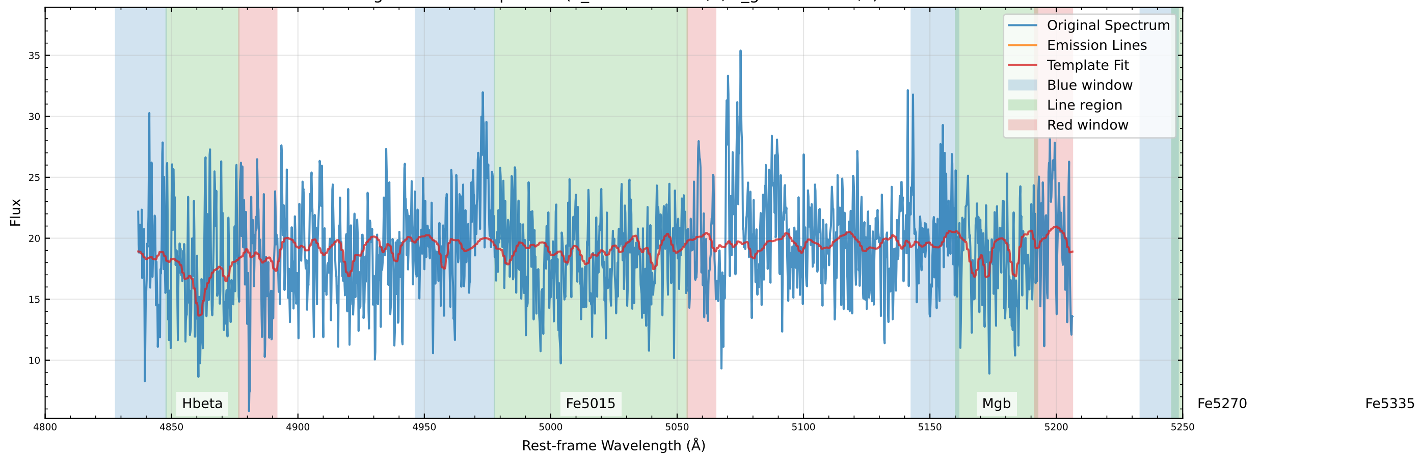
Original Data Comparison (v_star=-41.9 km/s, v_gas=11.3 km/s)
