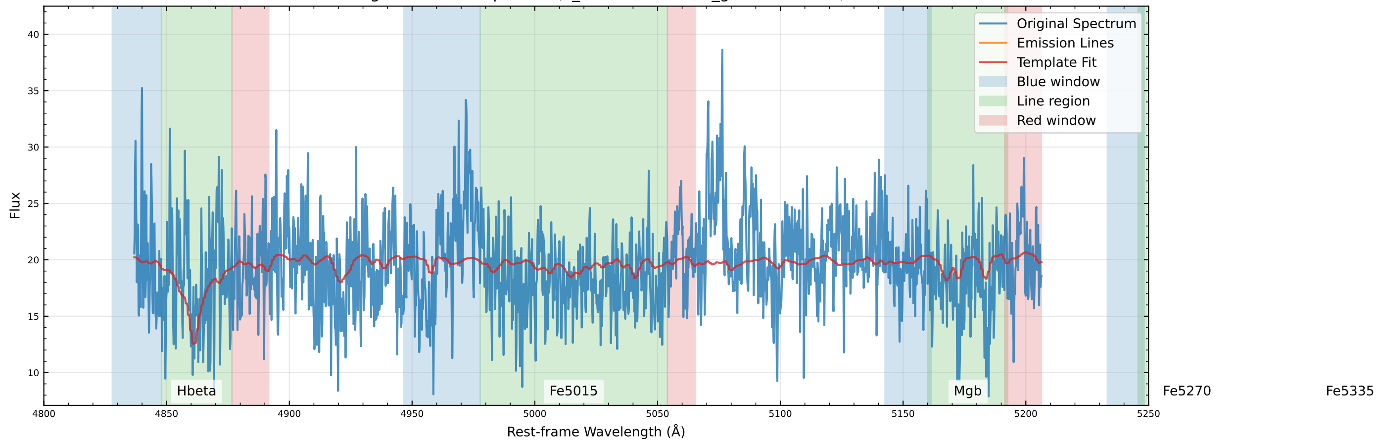
Original Data Comparison (v_star=5.2 km/s, v_gas=39.1 km/s)
