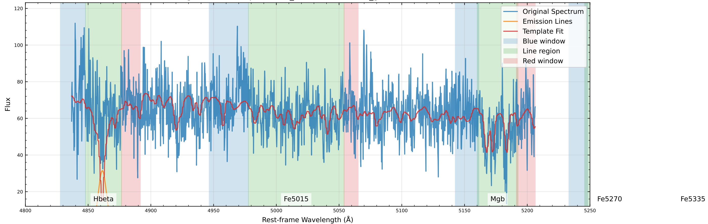
Original Data Comparison (v_star=-16.0 km/s, v_gas=-24.0 km/s)
