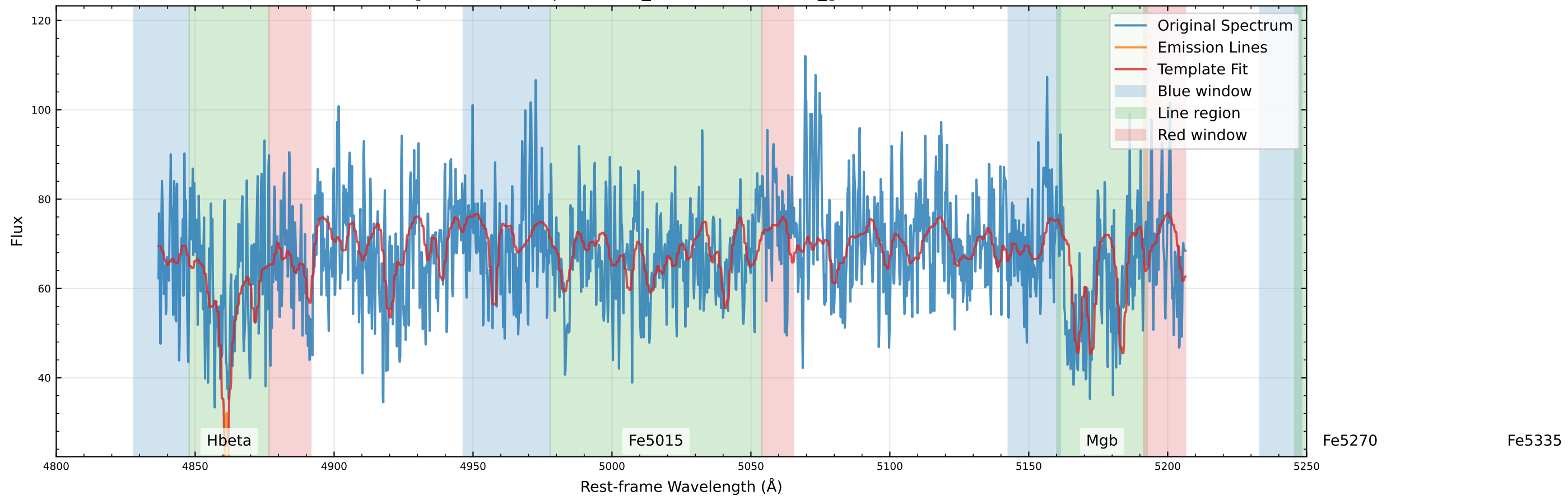
Original Data Comparison (v_star=-73.4 km/s, v_gas=-75.3 km/s)
