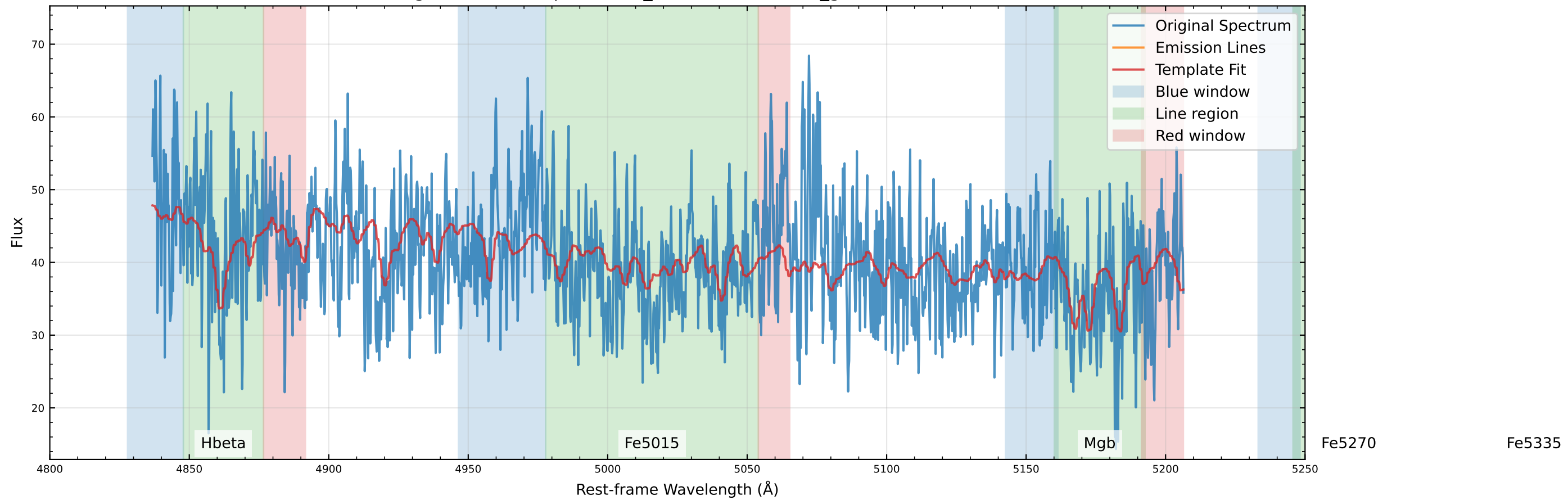
Original Data Comparison (v_star=-16.0 km/s, v_gas=-1.4 km/s)
