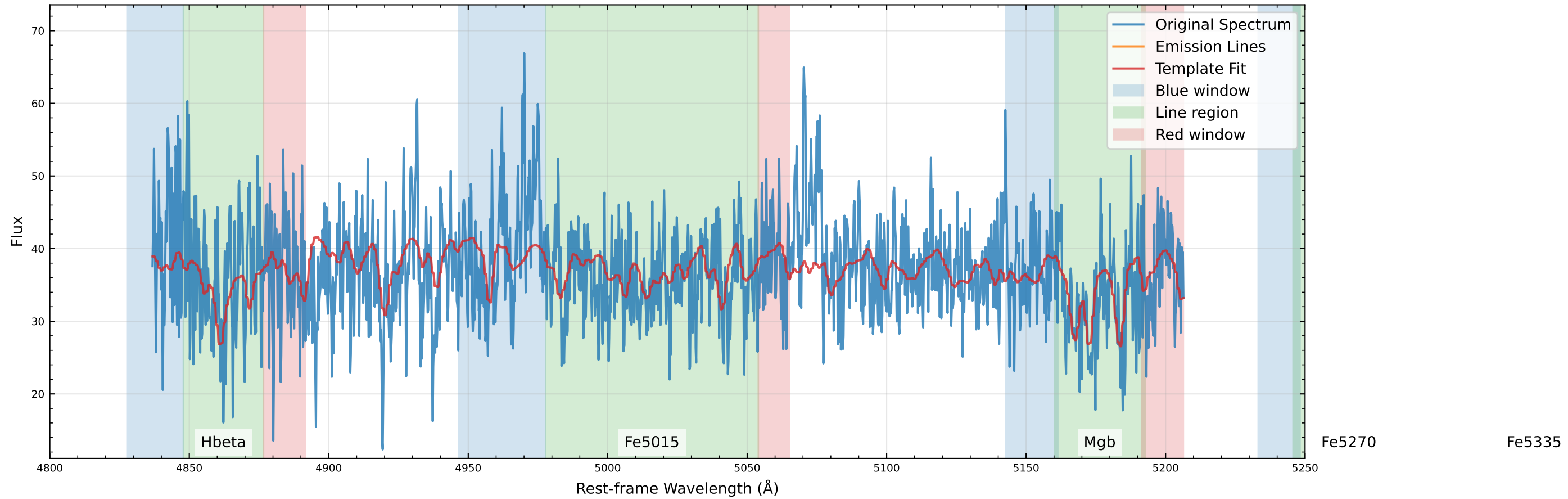
Original Data Comparison ( v_{\text{star}}=38.3 km/s, v_{\text{gas}}=338.3 km/s)
