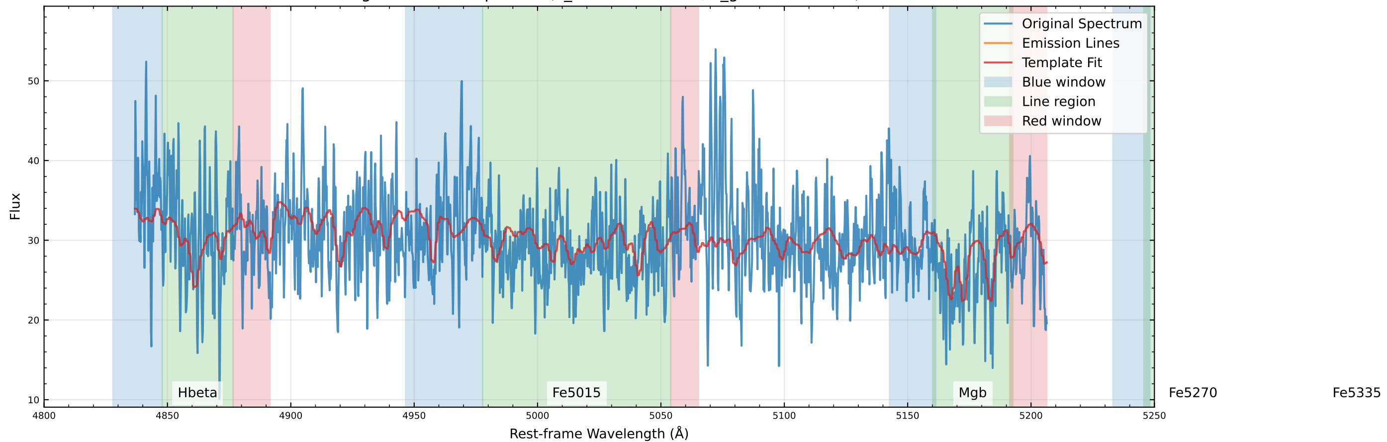
Original Data Comparison (v_star=-17.8 km/s, v_gas=-11.6 km/s)
