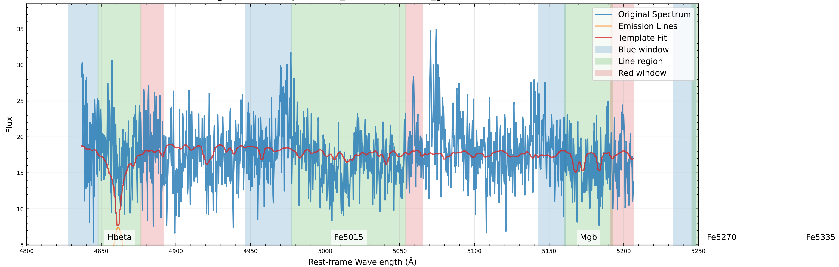
Original Data Comparison (v_star=36.5 km/s, v_gas=-111.8 km/s)
