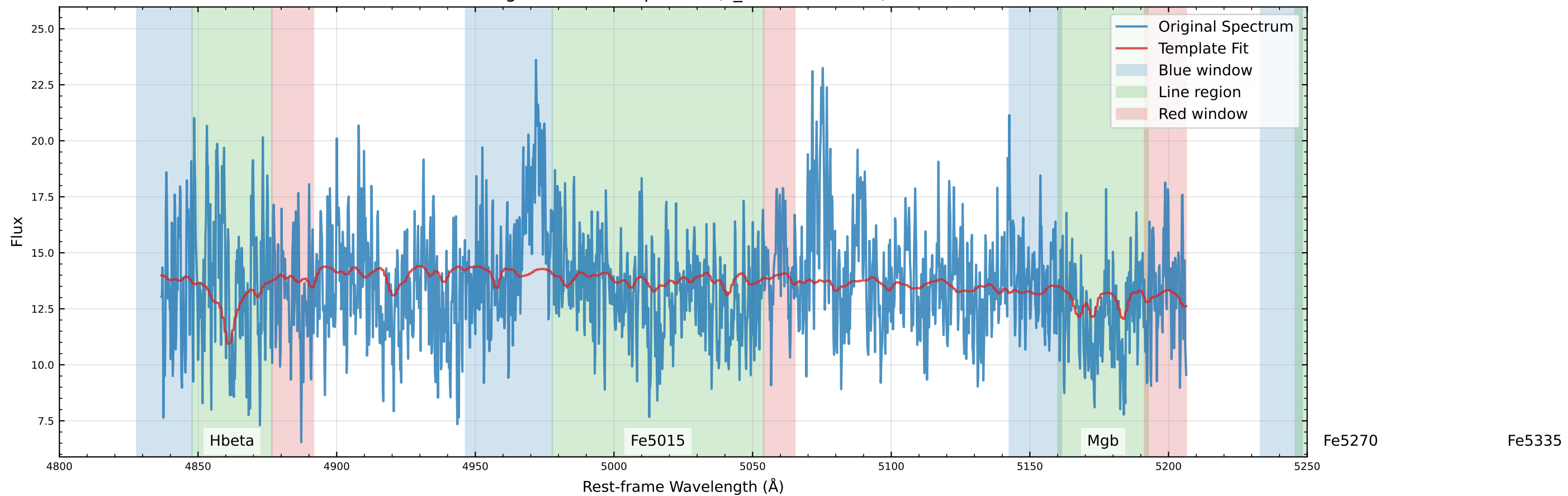
Original Data Comparison (v_star=52.8 km/s)
