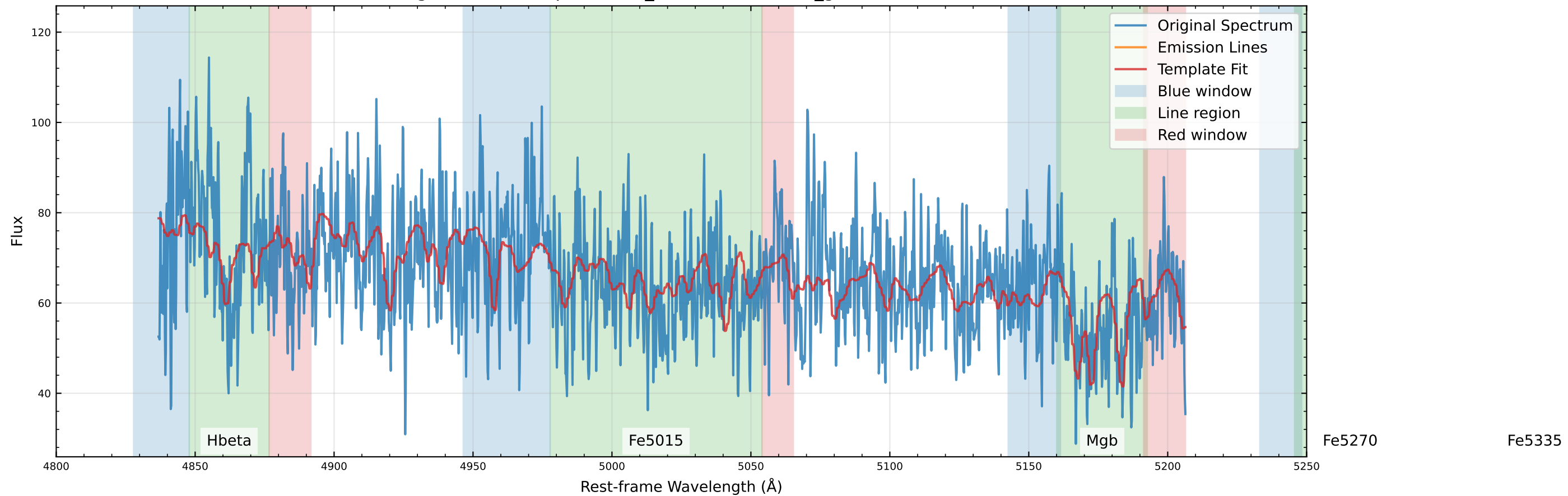
Original Data Comparison (v_star=21.8 km/s, v_gas=-93.5 km/s)
