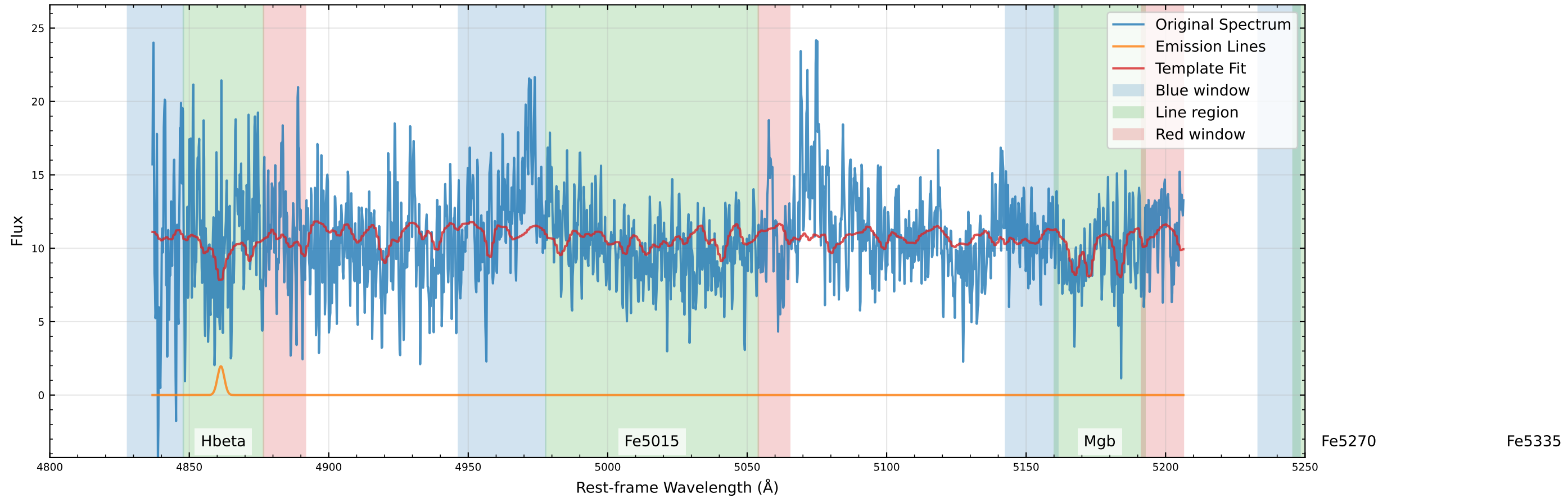
Original Data Comparison (v_star=-28.0 km/s, v_gas=0.1 km/s)
