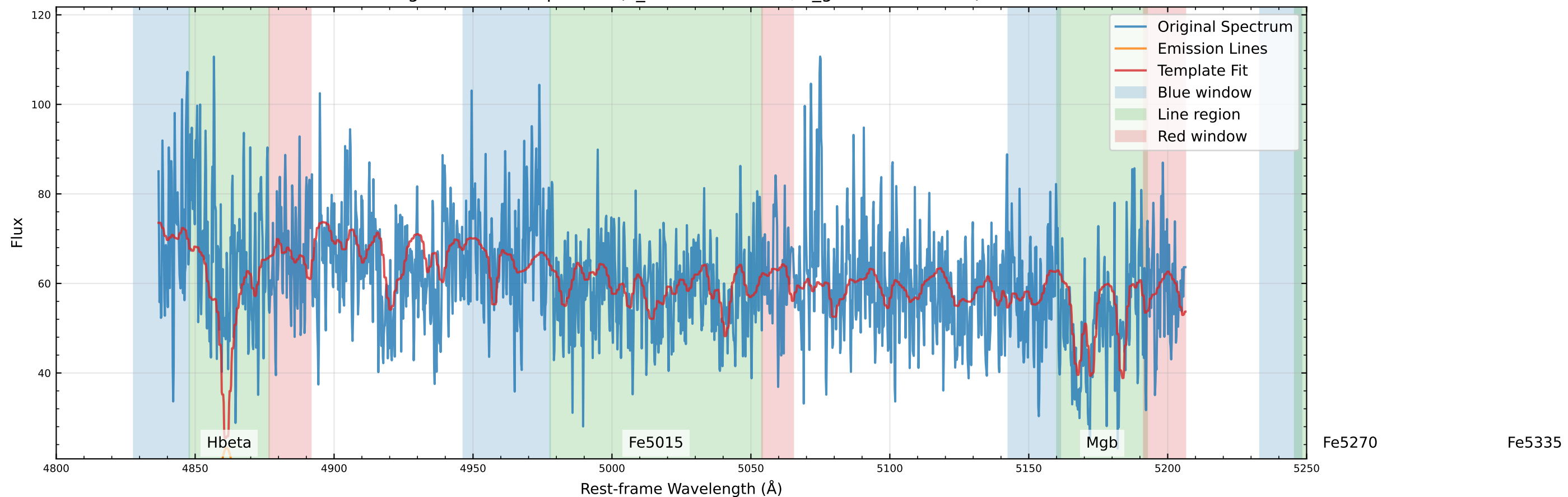
Original Data Comparison (v_star=-72.6 km/s, v_gas=-127.8 km/s)
