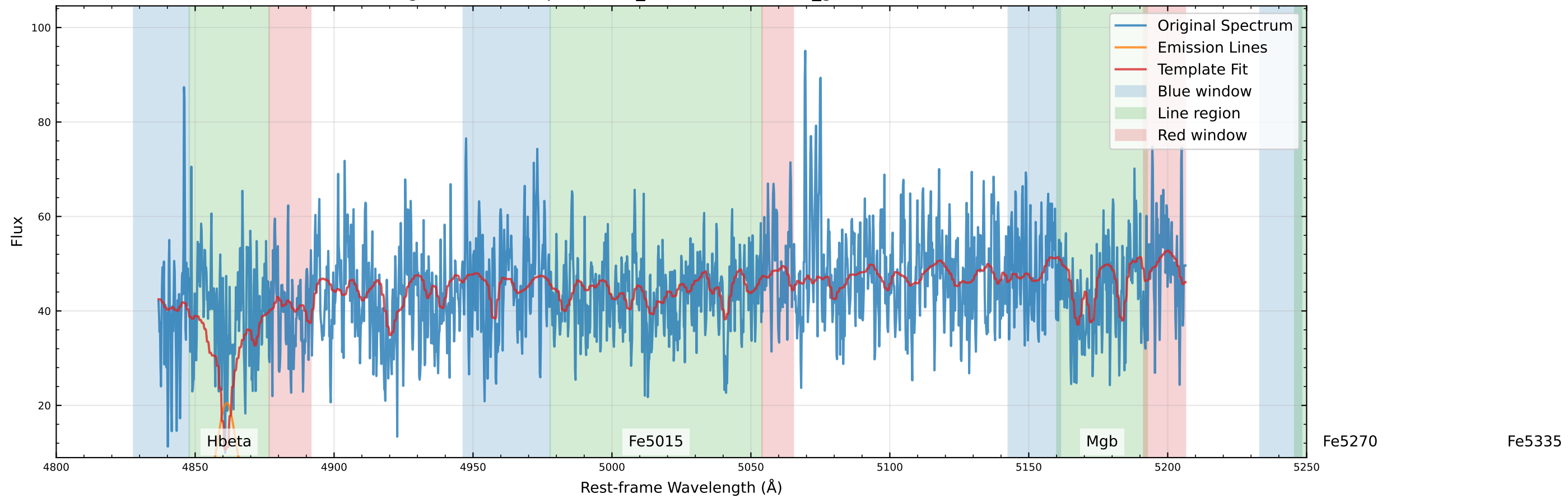
Original Data Comparison (v_star=-78.2 km/s, v_gas=-222.3 km/s)
