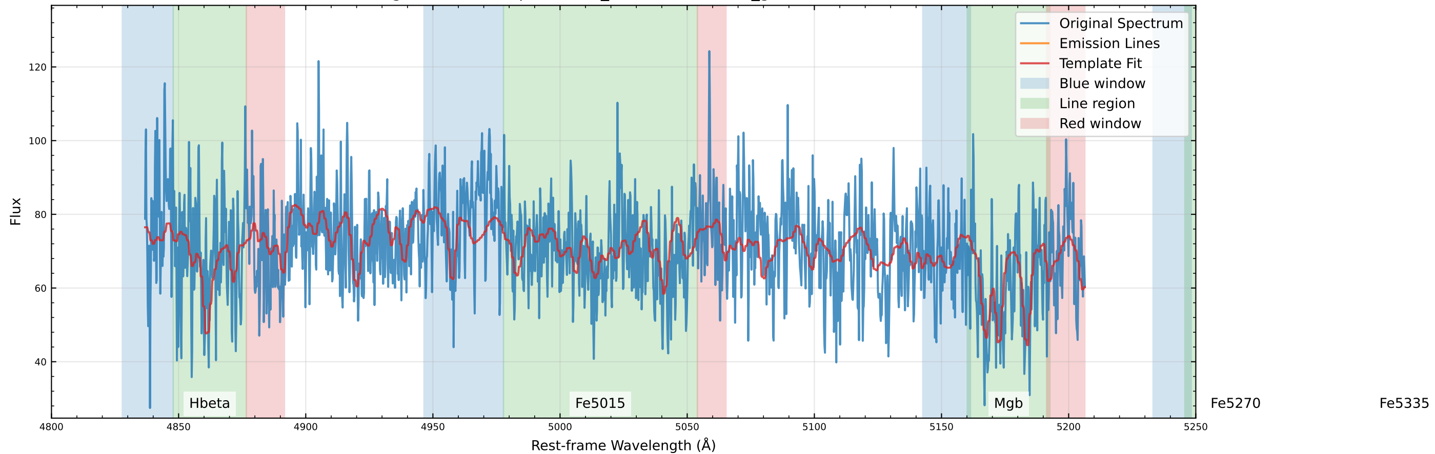
Original Data Comparison (v_star=-2.8 km/s, v_gas=2.1 km/s)
