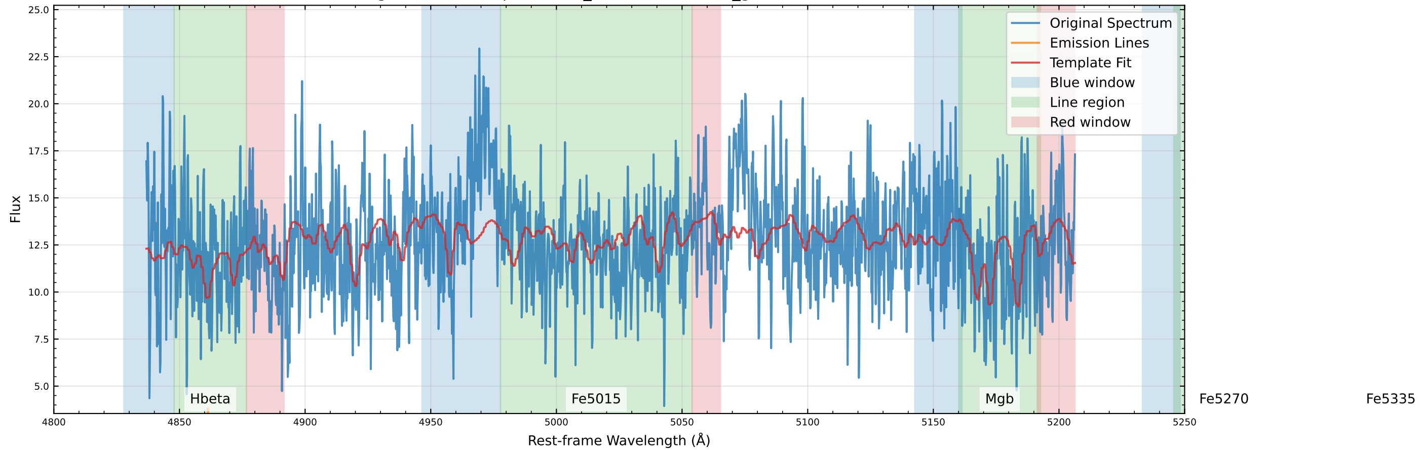
Original Data Comparison (v_star=-8.7 km/s, v_gas=-104.0 km/s)
